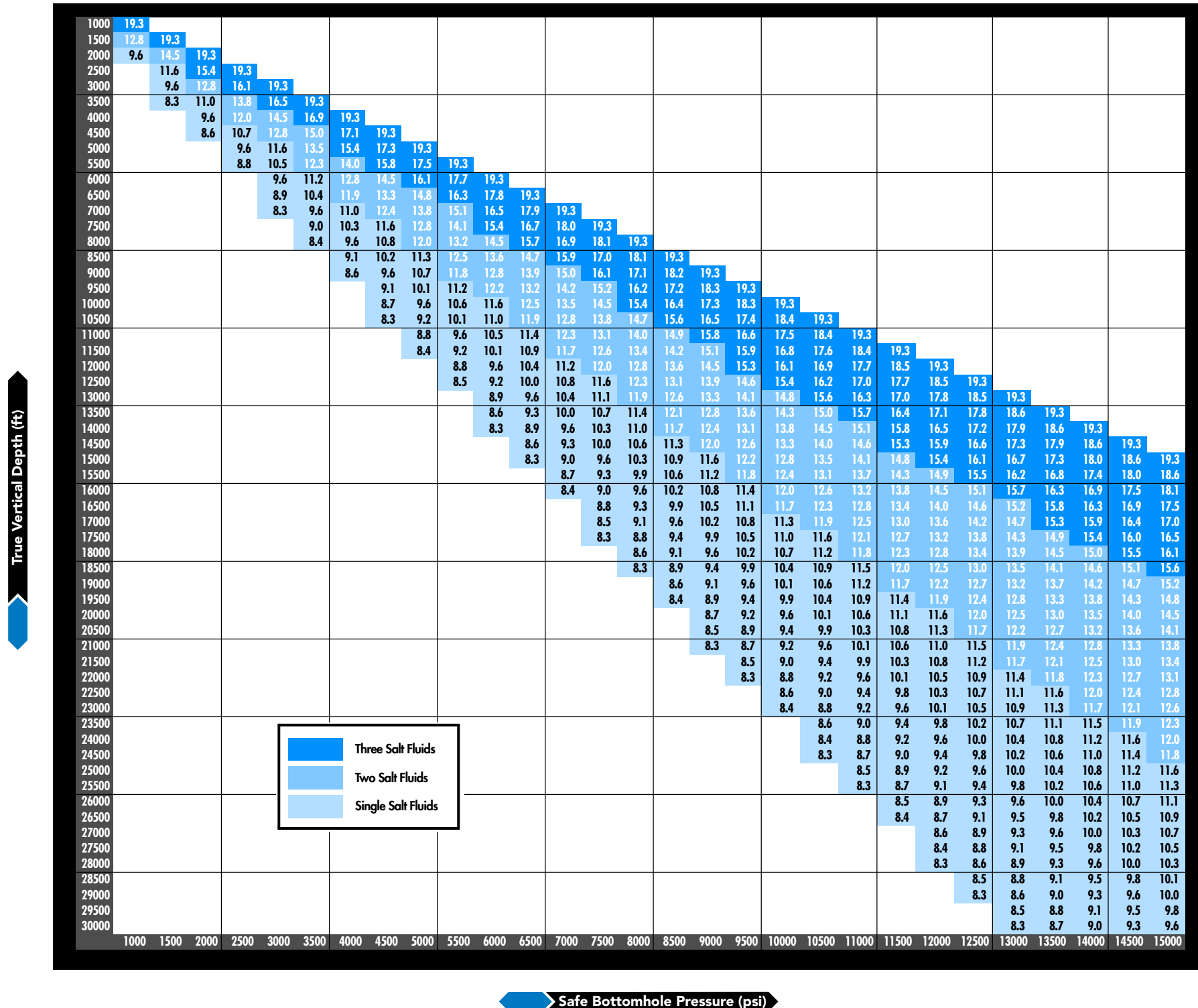
FIGURE 3. TVD-BHP Fluid Density Chart
